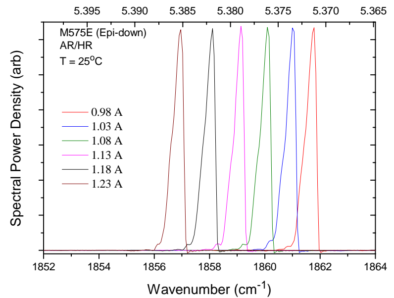
Wavelength ( \mu\text{m} )
