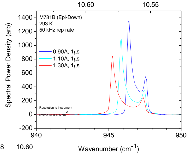
Emission Spectrum Wavelength ( \mu m)
